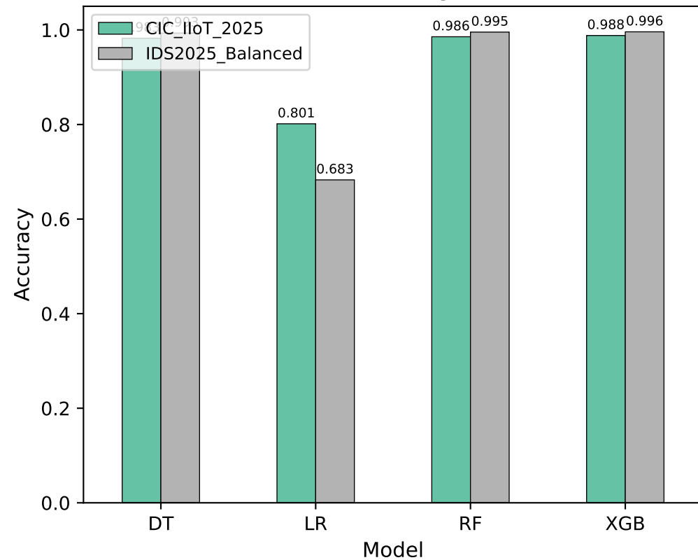
Accuracy
